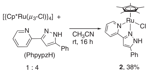
Scheme 3. Synthesis of protic pyrazole complex 2 .
