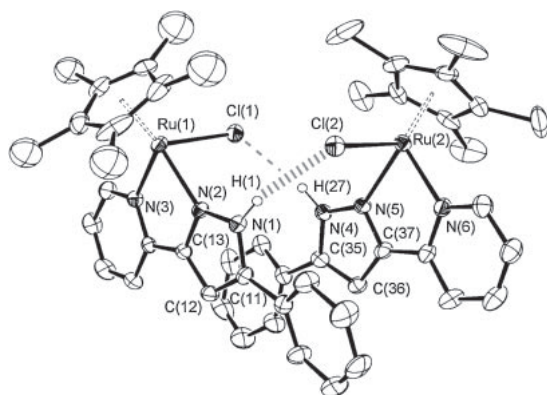
Figure 1. Crystal structure of 2 ·0.5THF with thermal ellipsoids at the 30% probability level. A pair of two crystallographically independent molecules is shown. Hydrogen atoms except for the NH protons, the minor component of the disordered Cp* ligand, and the solvated THF molecule are omitted for clarity.
