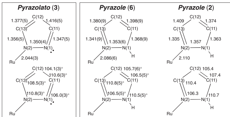
Figure 4. Bond distances (Å) and interior angles (deg) in the pyrazole ring of pyrazolato complex 3 and pyrazole complexes 6 and 2 . The values for 2 are averages of the two crystallographically independent molecules.
