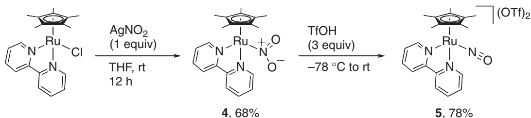
Scheme 5. Synthesis and protonation of nitro complex 4.
