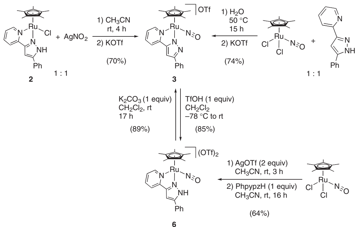
Scheme 4. Synthesis and reversible protonation of pyrazolato-nitrosyl complex 3 .
