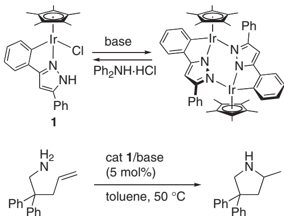
Scheme 2. Reversible dehydrochlorination of protic pyrazole complex 1 and intramolecular hydroamination of \omega -aminoalkene catalyzed by 1 .
