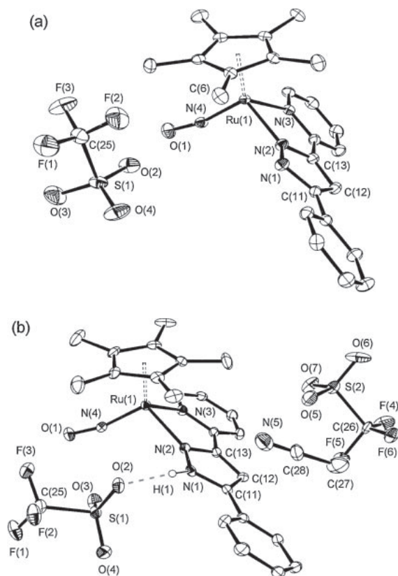
Figure 2. Crystal structures of 3 (a) and 6 ·CH 3 CN (b) with thermal ellipsoids at the 30% probability level. Hydrogen atoms except for the NH proton as well as the minor components of the disordered triflate anion are omitted for clarity.
