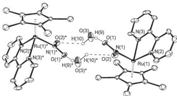
Figure 3. Crystal structure of 4 ·H 2 O with thermal ellipsoids at the 30% probability level. Only one of the two conformers of the disordered Cp* ligand is shown. Hydrogen atoms except for those in the solvated water molecule are omitted for clarity. Asterisks denote atomic position determined by crystallographic inversion center.
