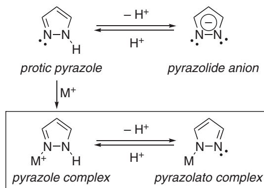
Scheme 1. Reversible deprotonation of uncoordinated and ligated protic pyrazole.
